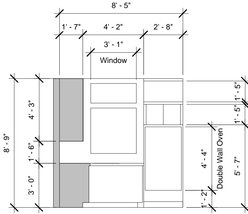
② End Wall Elevation 1/4" = 1'-0"
