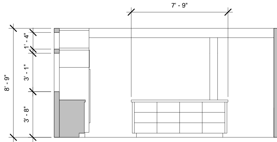
① Island Elevation 1/4" = 1'-0"
