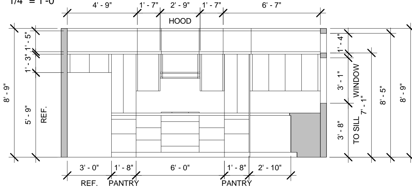
① Kitchen Wall Elevation 1/4" = 1'-0"
